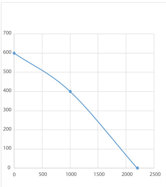
ComX-S 2500 / Air Flow Performance
